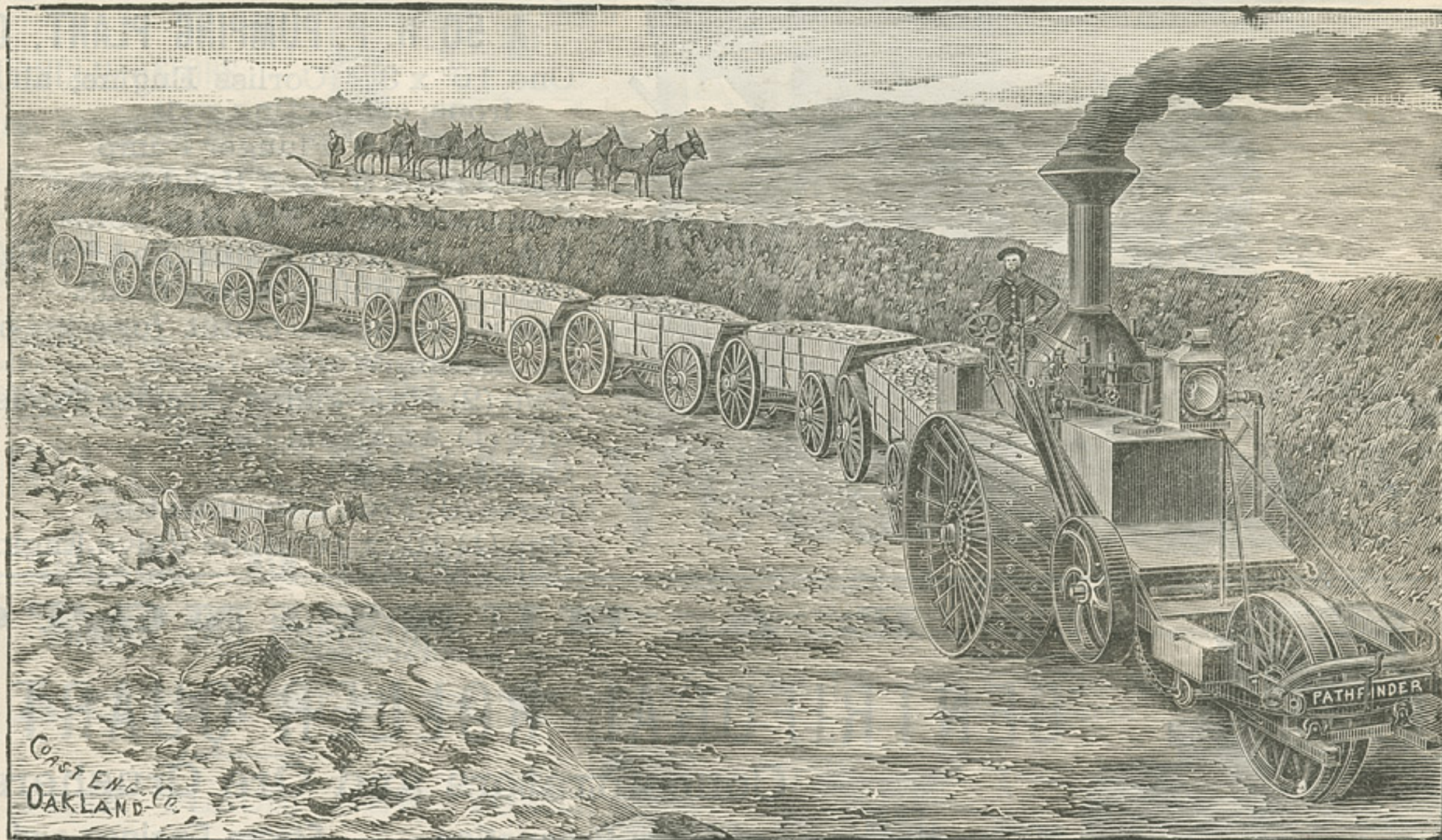
BEST'S TRACTION ENGINE HAULING GRAVEL IN SACRAMENTO.
